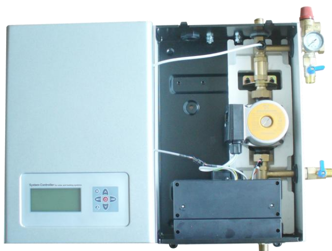
SR961S single line pump station
