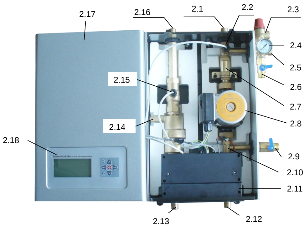
SR962S double line pump station
